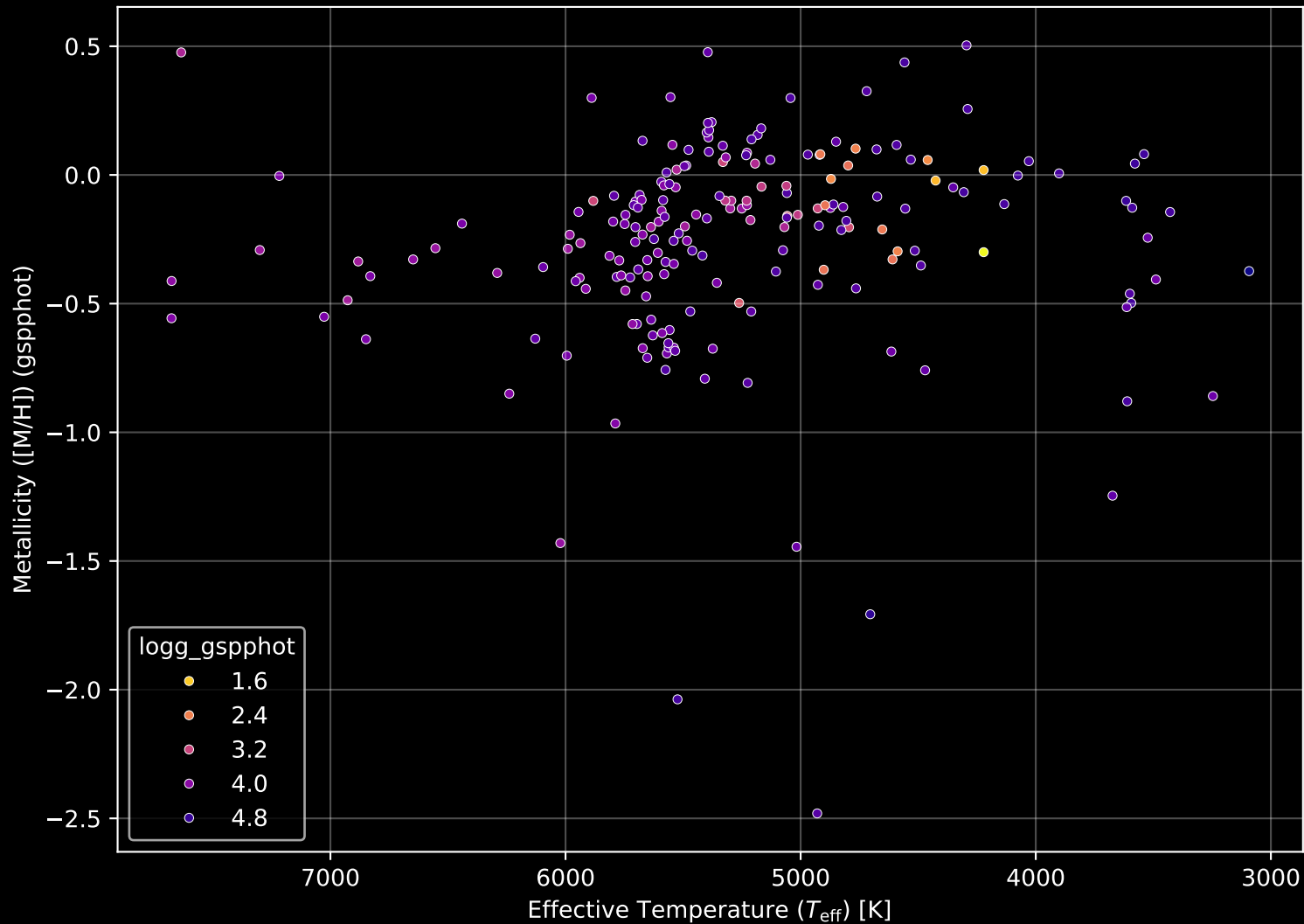
APOGEE DR17 Field: [130-48_MGA] Stellar Population Parameters (n= 200)
