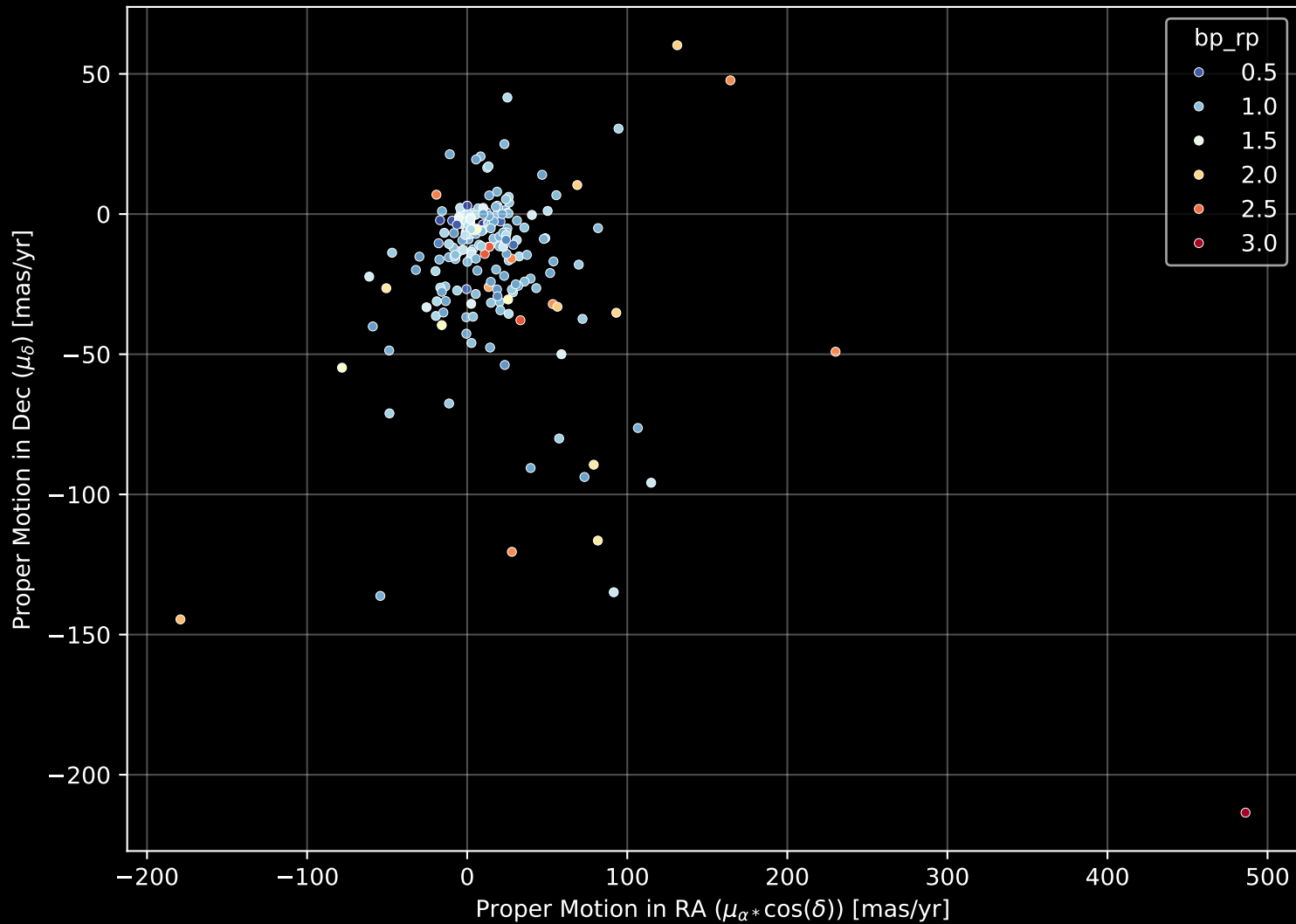
APOGEE DR17 Field: [130-48_MGA] Proper Motion Diagram (n= 200)
