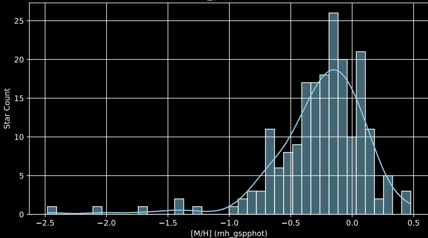
APOGEE DR17 Field: [130-48_MGA [M/H] (mh_gspphot) (n= 199)
