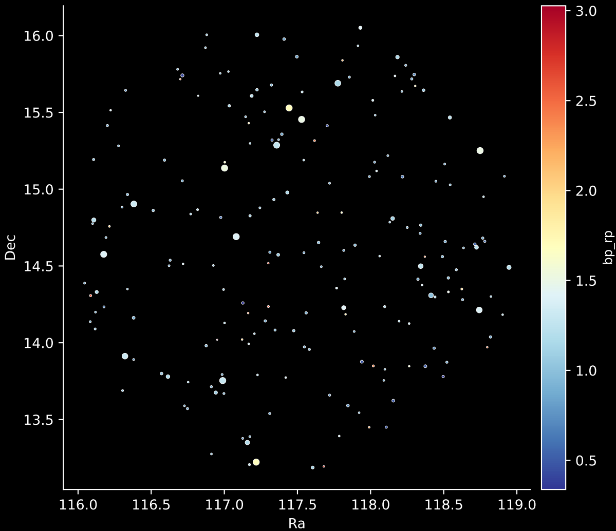
APOGEE DR17 Field: [130-48_MGA] Stars: 200
